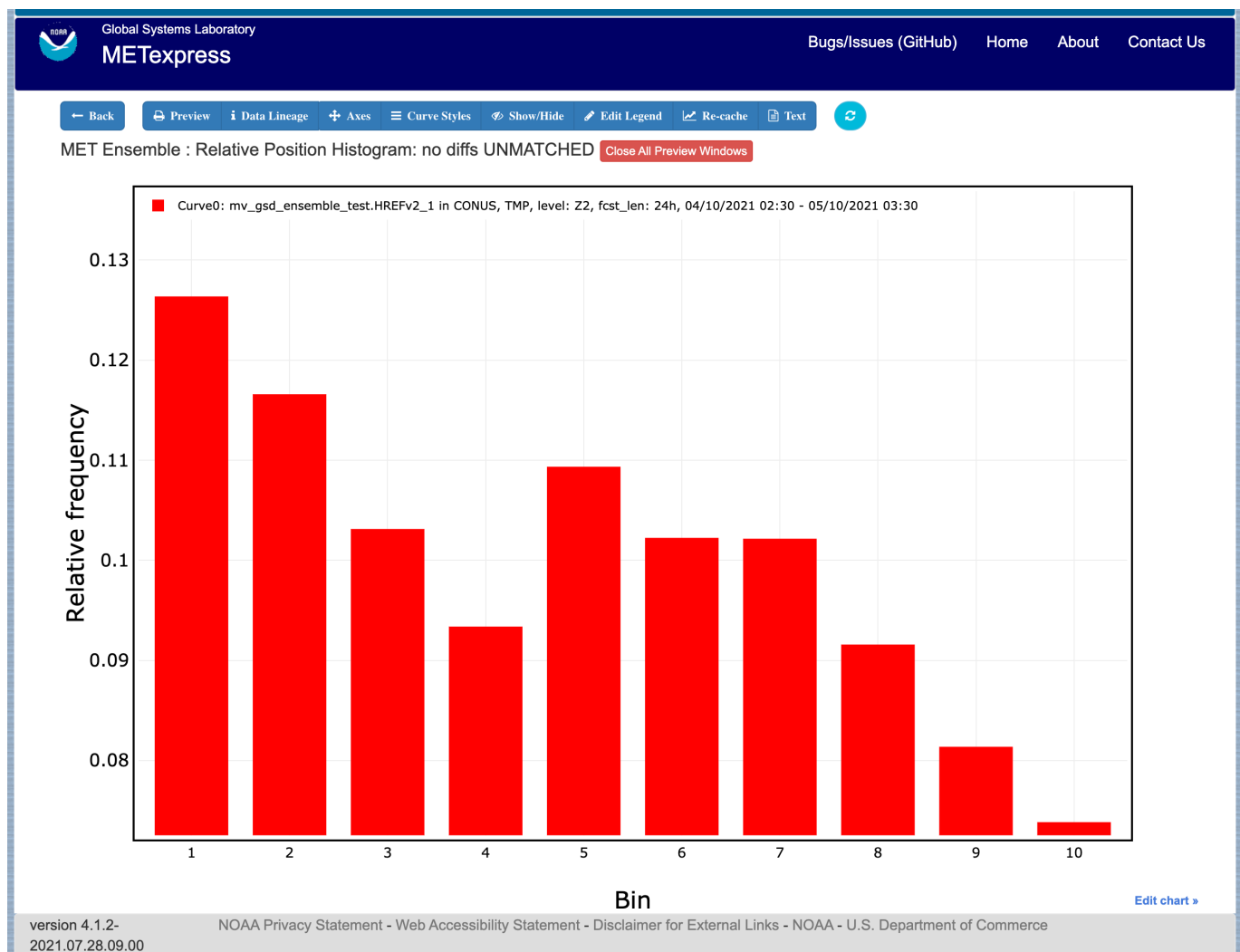
Figure 3.15: Ensemble Histogram plot type with Histogram Type of Relative Position Histogram
