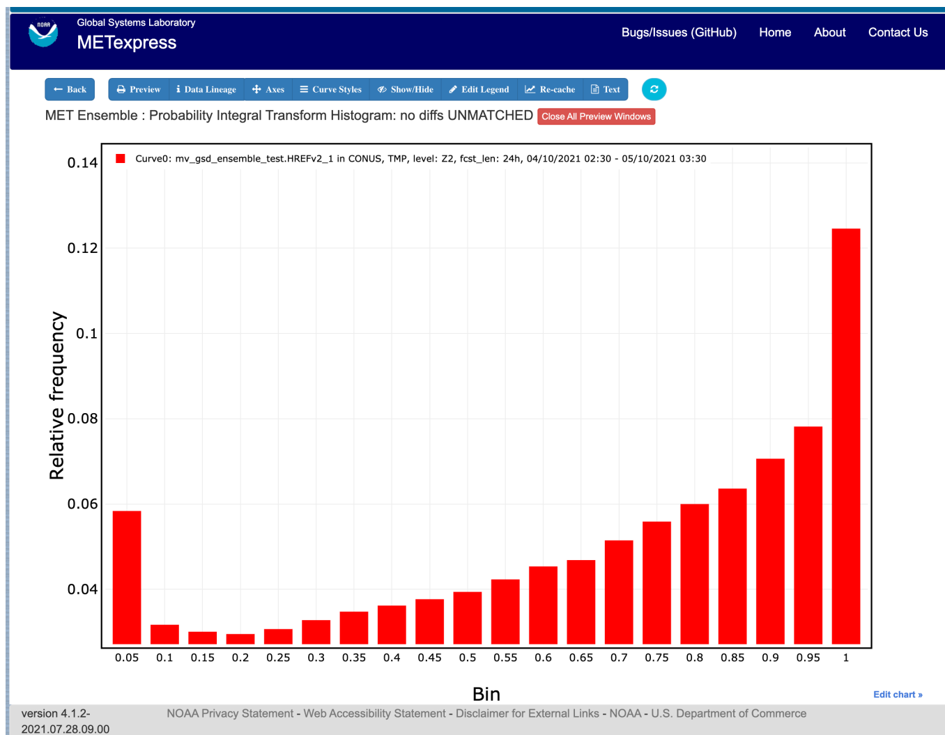
Figure 3.14: Ensemble Histogram plot type with Histogram Type of Probability Integral Transform Histogram.
