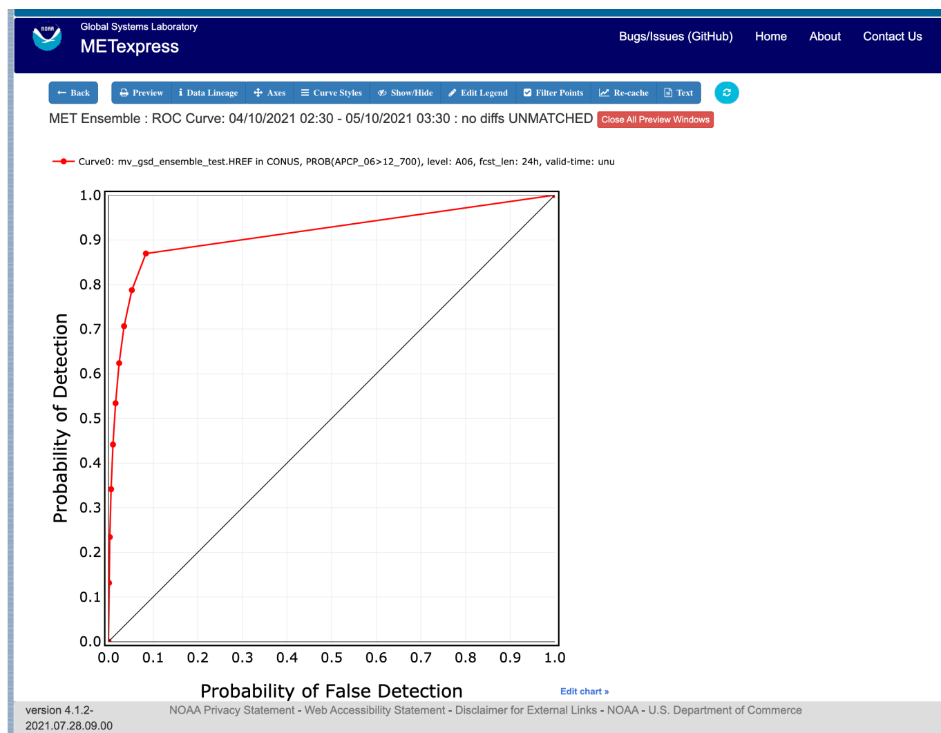
Figure 3.17: Ensemble app ROC plot for the same data set defined in Figure 3.16.
