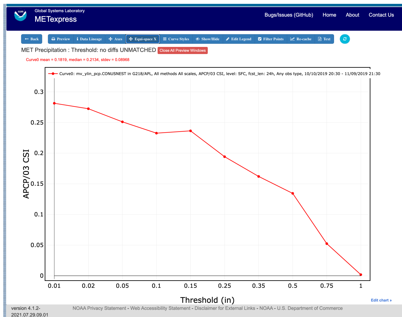
Figure 3.20: Threshold plot in the Precipitation app produced from selections in Figure 3.19
