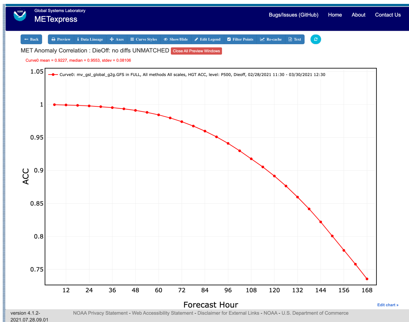
Figure 3.3: Anomaly Correlation DieOff plot
