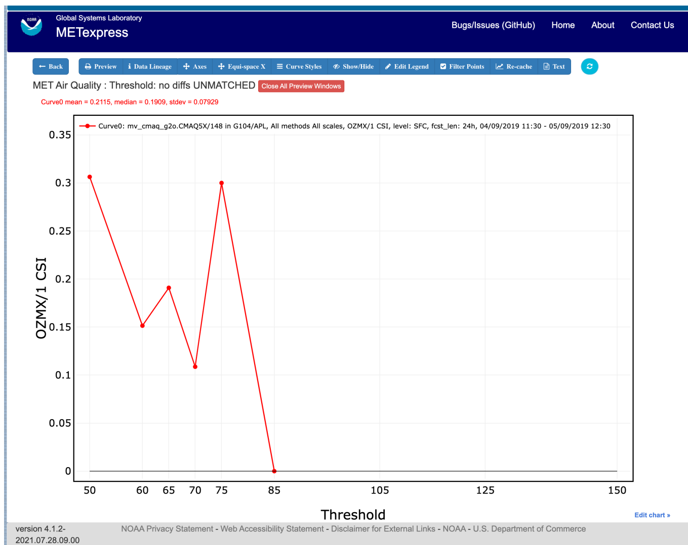
Figure 3.11: Air Quality app Threshold plot
