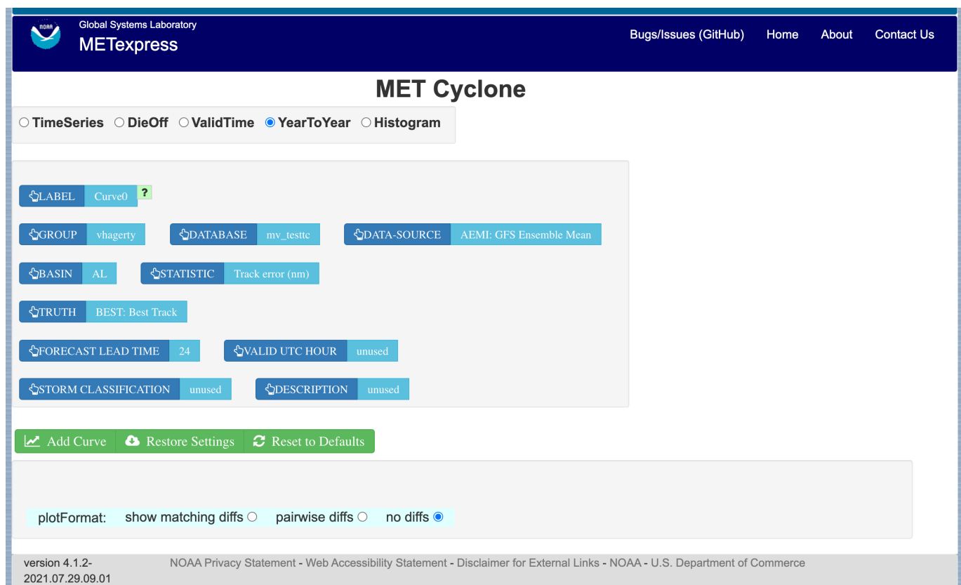
Figure 3.22: User interface screen for a YearToYear plot in the Cyclone app
