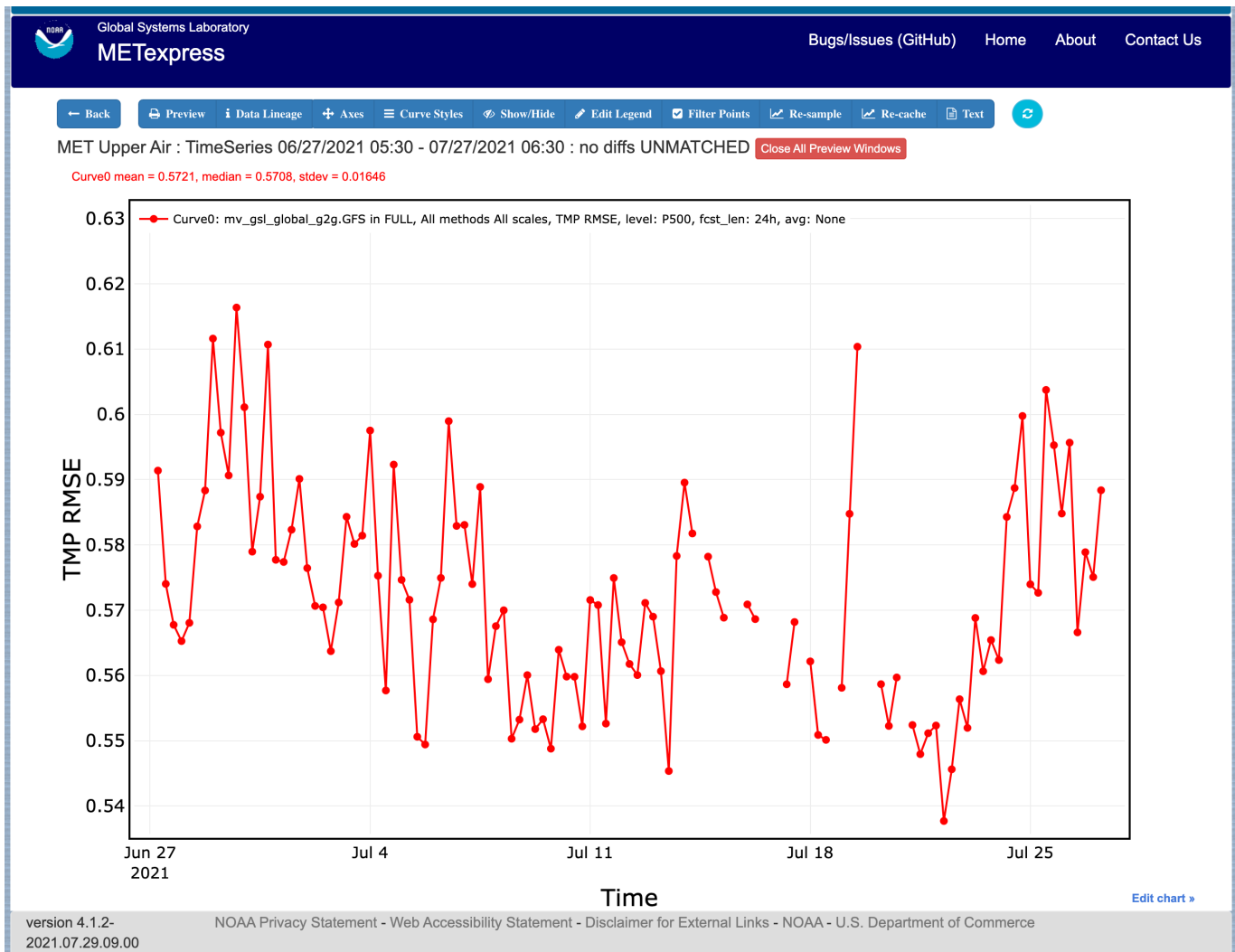
Figure 2.6: Plot of Time Series for a single curve with default values
