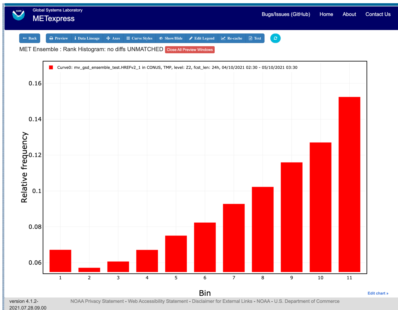
Figure 3.13: Ensemble Histogram plot type with Histogram Type of Rank Histogram.
