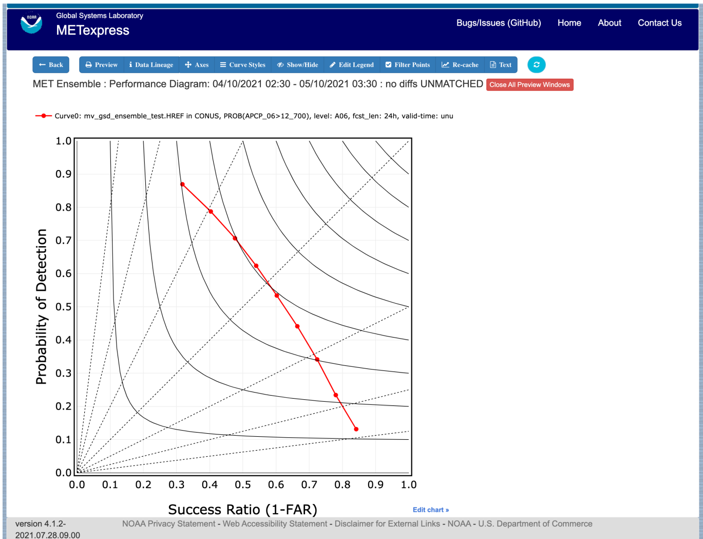
Figure 3.18: Ensemble app Performance Diagram for the same data set defined in Figure 3.16 .
