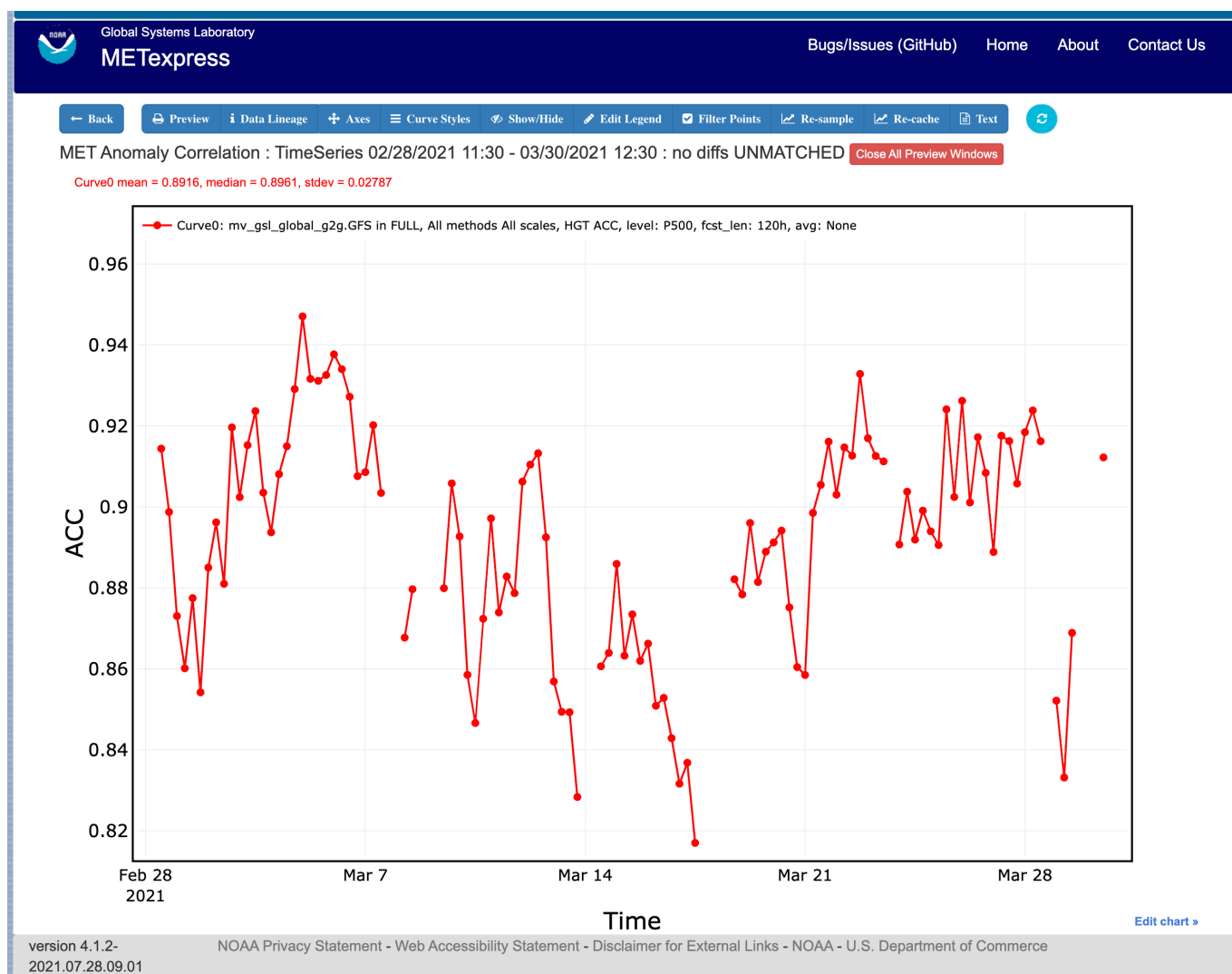
Figure 3.8: Anomaly Correlation sample plot.
