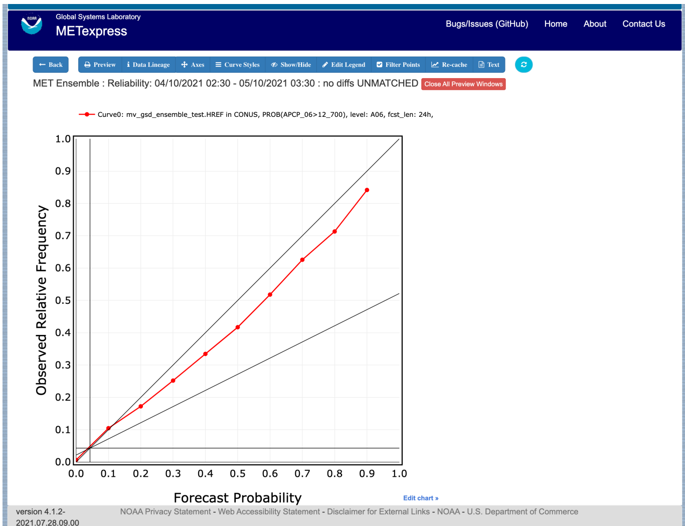
Figure 3.16: Ensemble app Reliability plot. The 1:1 diagonal gray line represents perfect skill between forecast probability and observation frequency. The diagonal line with the lower slope indicates the point above which the forecast becomes more skillful than climatology, and the vertical and horizontal lines indicate climatology.
