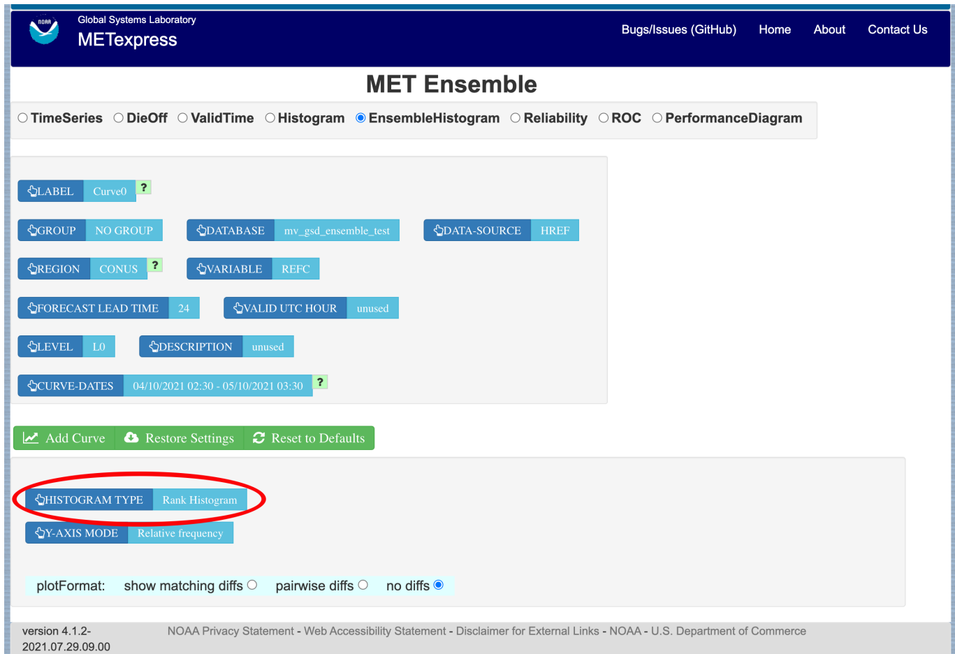
Figure 5.23: The Ensemble app user interface for Ensemble Histogram plots. Note the selector for Histogram Type which is unique to this plot type.
